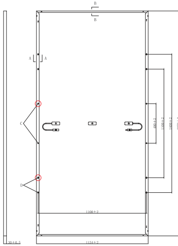
Mounting Hole
